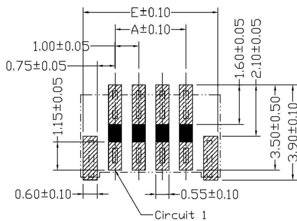
P. C. B LAYOUT
