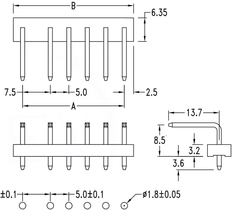
P. C. Board Hole Dimensions
