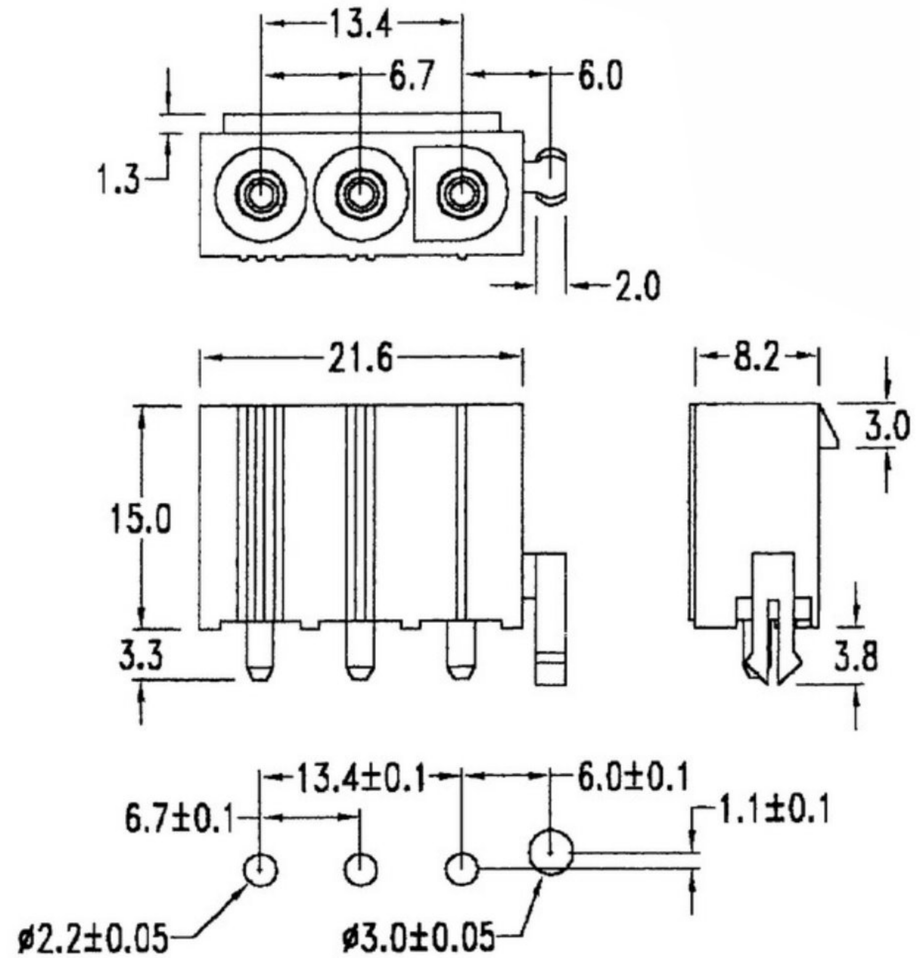
P. C. board hole dimensions
