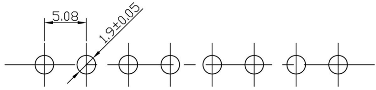
RECOMMENDED P.C. BOARD HOLE DIM.
