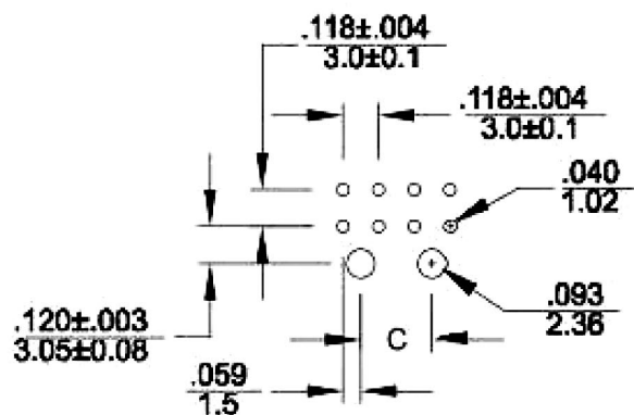
PCB Layout: Component side
