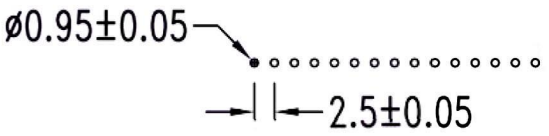
P. C. board hole dimensions
