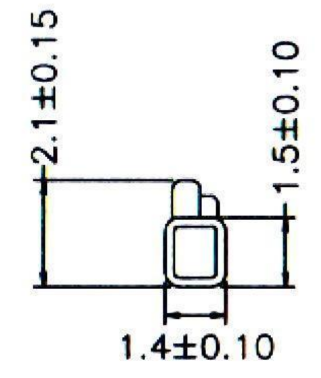
Section C-C
