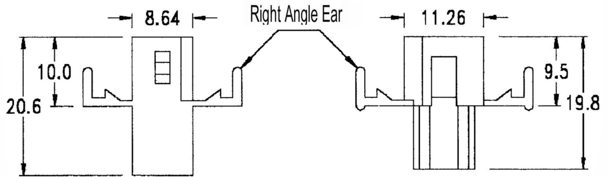
Male Housing
