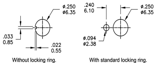
PANEL MOUNTING
