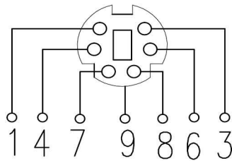
SCHEMATIC DIAGRAM
