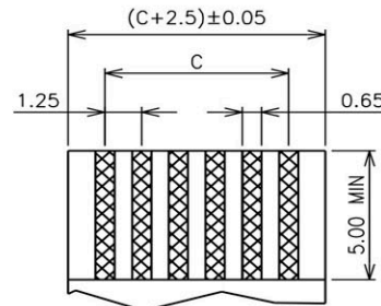
FPC/FFC T=0.30±0.05
