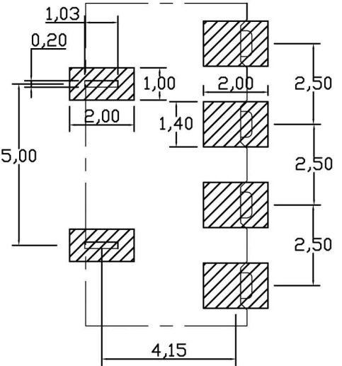
RECOMMENDED PCB LAYOUT TOP VIEW (. XX ± 0.05)
