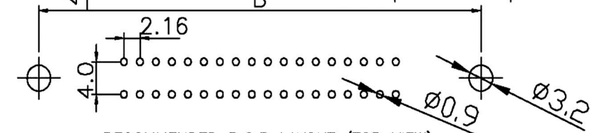
RECOMMENDED P.C.B LAYOUT (TOP VIEW) TOLERANCES: ±0.10mm
