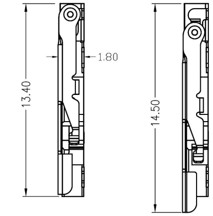
SLIDE SHELL OPEN SLIDE SHELL LOCK
