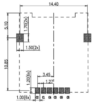
PCB LAYOUT
