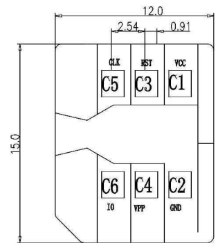
MICRO SIM
