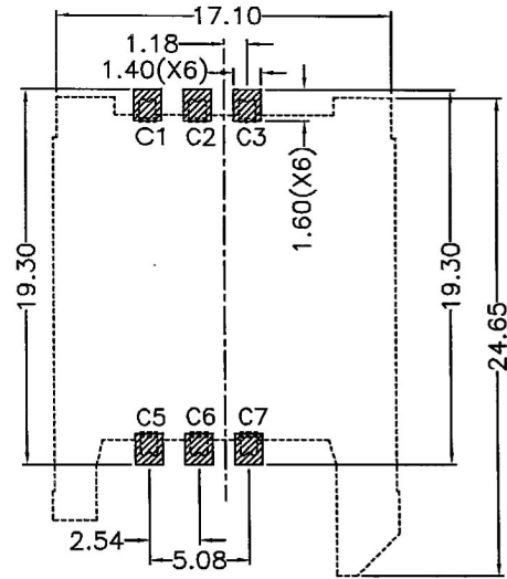
RECOMMENDED P.C.B LAYOUT COMPONENT SIDE(TOLERANCE ±0.05)
