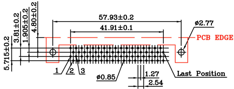
PCB Layout (B)
