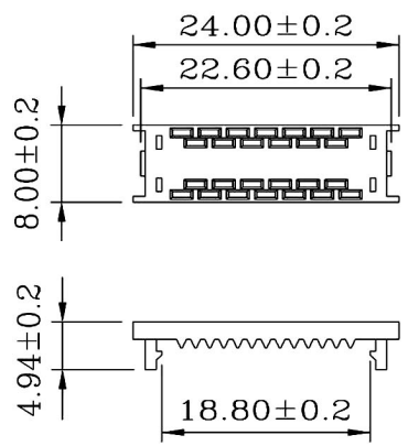
Termination Cover (1 Places)
