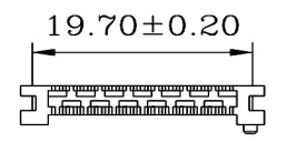
Wire Holder=0.62mm (2 Places) *WIRE HOLDER:28Awg
