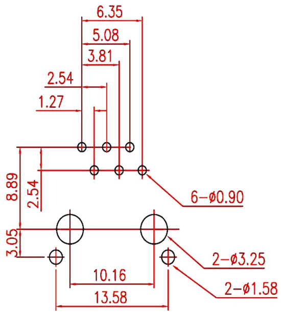
PCB Layout
