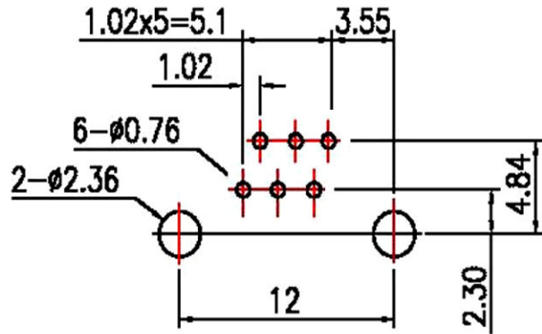
PCB Layout
