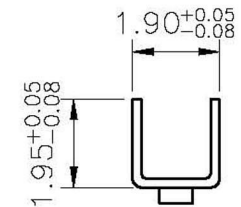
SEC:C-C
