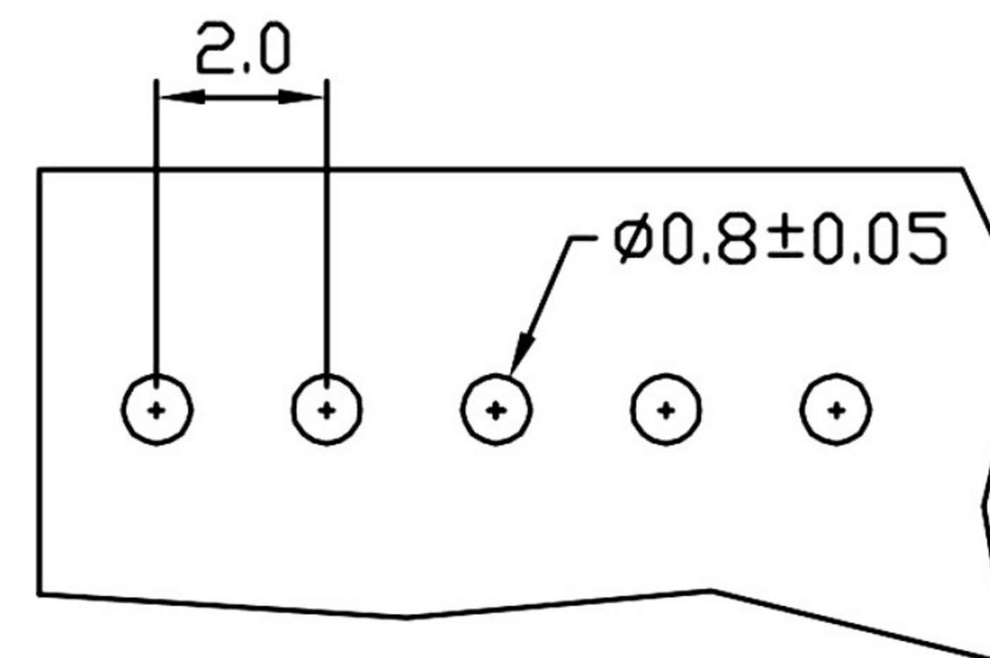
P.C. BOARD LAYOUT
