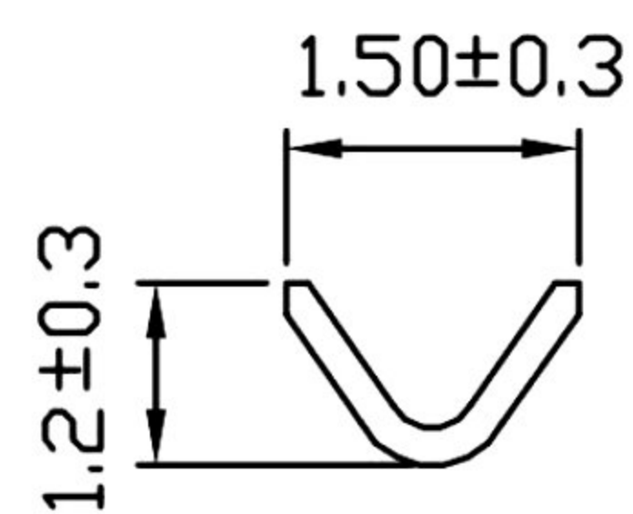
Section B-B'
