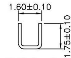
SEC:C-C
